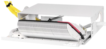
FIST-GSS3 Fiber Splice Panel, 3RU, 15 in, gray
